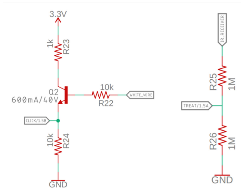
Figure 3: (Left) Transistor to detect the RF remote being activated, (Right) resistor divider circuit to read the IR receiver output voltage. Note: “WHITE WIRE” is the hardware connection to the RF receiver; “CLICK” is the output signal for the RF receiver; “TREAT” is the voltage reading from the output of the IR receiver.
